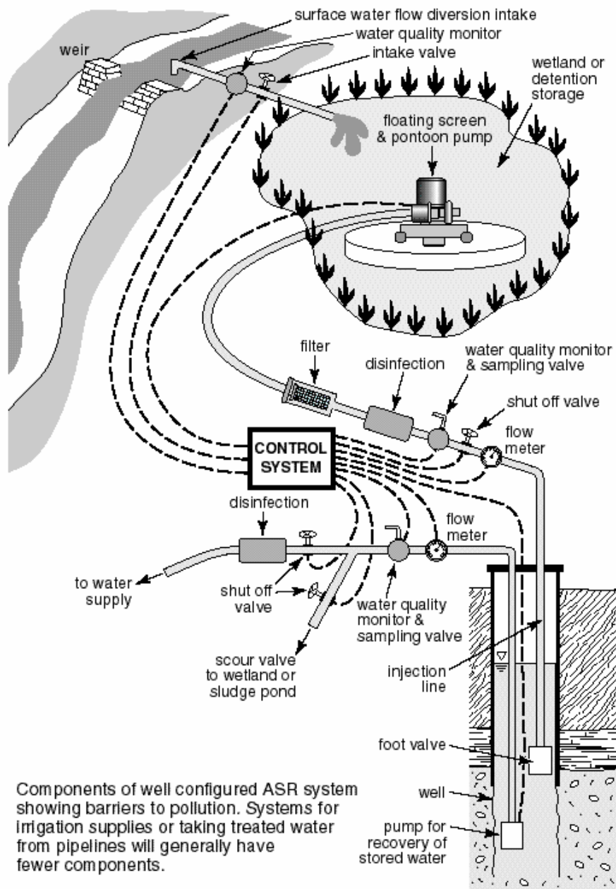
Figure 12.1 Components of a well-configured ASR system (diagram CSIRO Land and Water)
