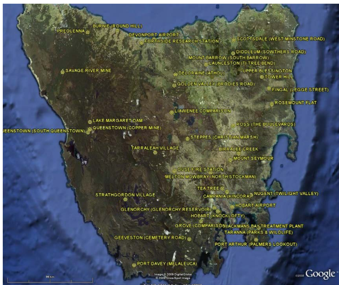
Figure A.1. BOM pluviographic rainfall stations
